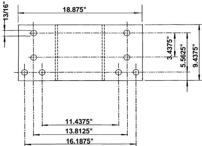
Girder/Endtruck Bolt Pattern
