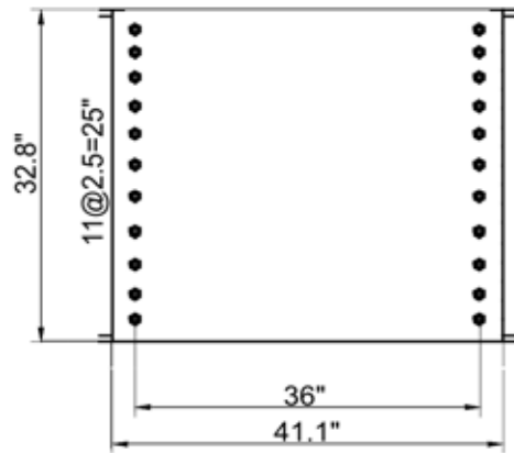
Endtruck/Girder Connection Plate
